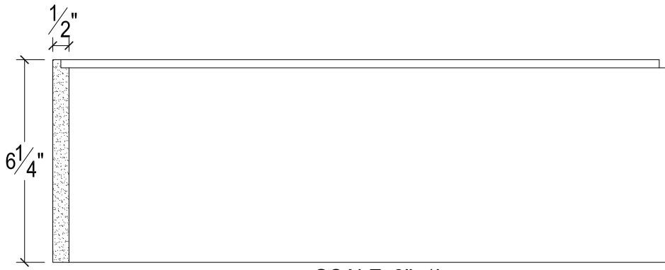
SCALE :3"=1'
