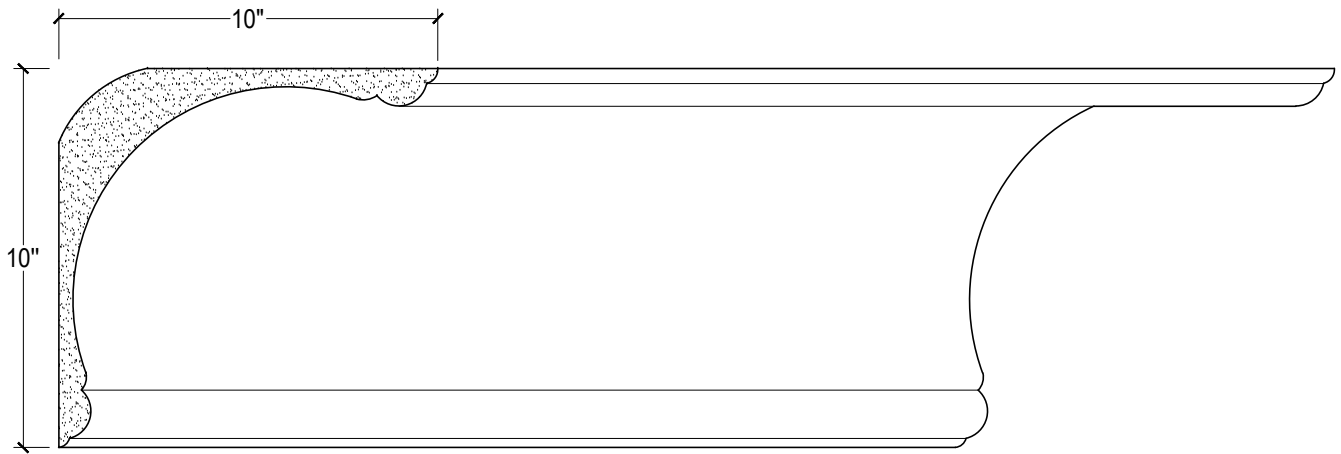
SCALE :4"=1'
