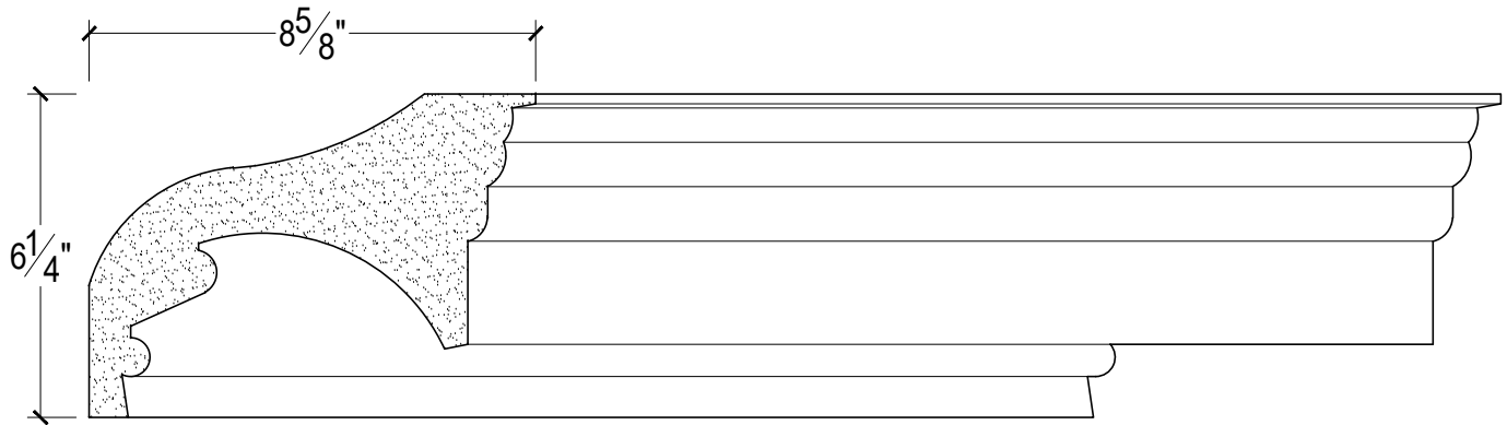
SCALE :3"=1'
