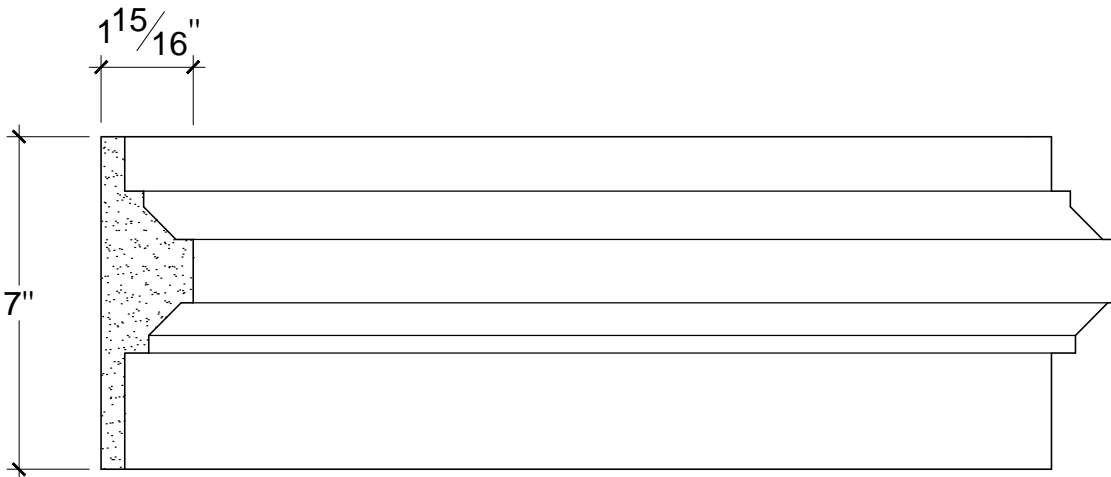
SCALE :3"=1'
